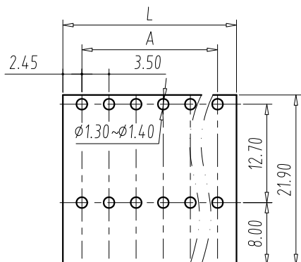
PCB LAYOUT S=1.5:1
