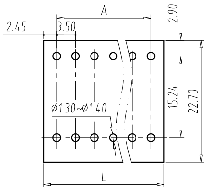
PCB LAYOUT S=1.5:1
