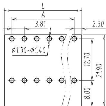
PCB LAYOUT S=1.5:1
