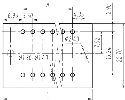
PCB LAYOUT S=1.5:1
