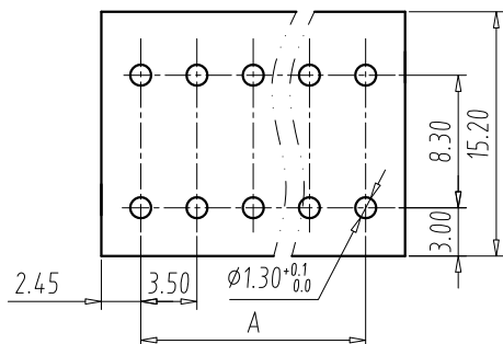
PCB LAYOUT S=1.5:1
