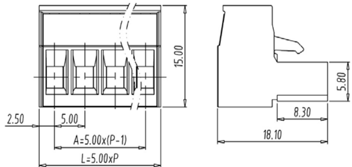
■ 图示(Pic. shown) : TLPS-200V-1066-06P-G12S
