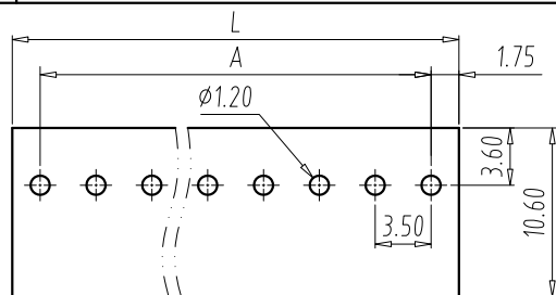
PCB LAYOUT S=2:1
