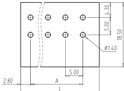
PCB LAYOUT S=2:1
